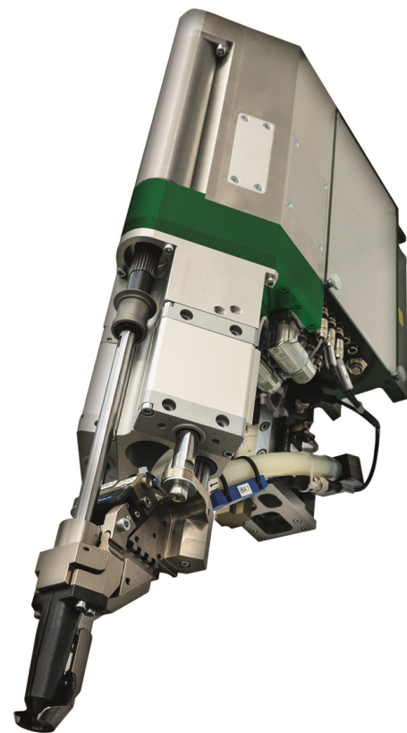
ADAPTIVE DFS
